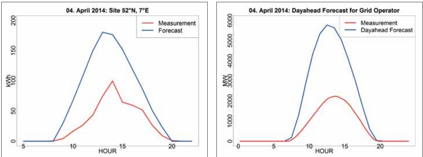
Figure 1. The difference between forecast and actual production during a Saharan dust outbreak for a single site (left) and at a grid level
