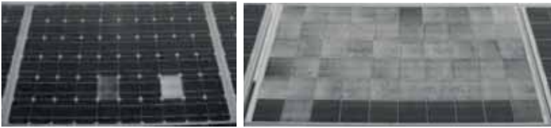
Figure 3: electroluminescence images from PID-affected modules in field: 'surface' PID (left) and 'frame' PID (right) depending on different leakage current distribution in PV modules [1]
