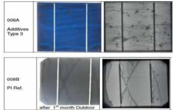
Figure 6. Different visual appearance of snail trails depending on additives in EVA [2]
