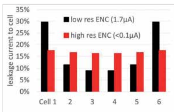
Figure 2. Leakage current distribution depending on kind of encapsulation material (high volume resistivity ( 10^{15} \Omega\text{cm} ) versus low volume resistivity ( 10^{13} \Omega\text{cm} )) [1]
