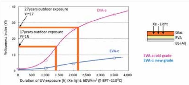
Figure 4. Different trends for the yellowness index for two different EVA formulations
